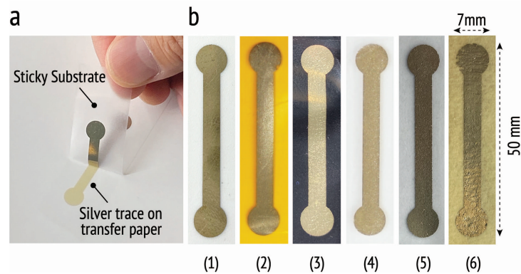
Fig. 3. Silver traces transferred to different substrates. (a) Transfer process. (b) Successfully transferred conductive patterns on various substrates: (1) Scotch tape (3M Scotch 810), (2) polyimide electrical tape (3M 1205), (3) vinyl insulation tape (3M Super 33+), (4) water soluble wave soldering tape (3M 5414), (5) Scotch removable tape (3M Scotch 811), (6) masking tape (3M Scotch 234).
