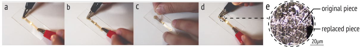
Fig. 5. (a) Silver trace is transferred onto PDMS and connected with LED. (b) Part of the trace is removed. (c) Recovering the damaged portion with a new silver trace. (d) The silver trace is recovered. (e) Microscopic image of the edge between the original and the replaced silver trace.
