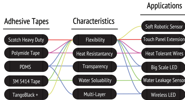
Fig. 8. Application Overview
