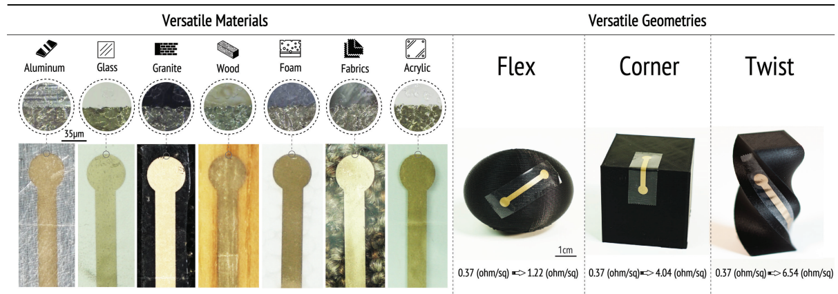
Fig. 6. Silver traces transferred onto different materials and geometries.
