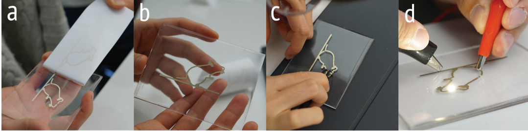
Fig. 10. Workshop Results: Participants completing fabrication steps from transferring the mouse pattern to PDMS sheet, mounting the LED with conductive Epoxy, and lighting it up with DC power supply.
