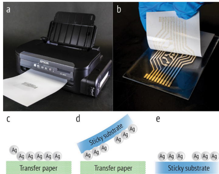
Fig. 2. Overview of Silver Tape. Conductive patterns are (a) printed on transfer paper, (b) peeled off and transferred by hand. (c-e) Schematics of the transfer process of silver nanoparticles from transfer paper to a sticky substrate.
