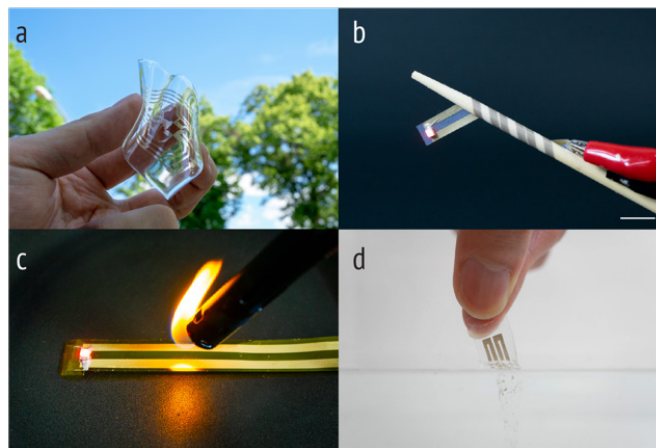
Fig. 1. Different functions enabled by different substrates with unique properties, including (a) transparency, (b) conformability, (c) fire tolerance, and (d) water solubility.
