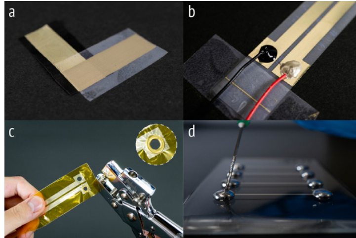
Fig. 4. Connection methods. (a) Pasting two sticky substrates using their own adhesive force. (b) Conductive paste/epoxy. (c) Pierce punch to make a stable, solderable connection. (d) Temporary liquid metal connection mainly for measurement.
