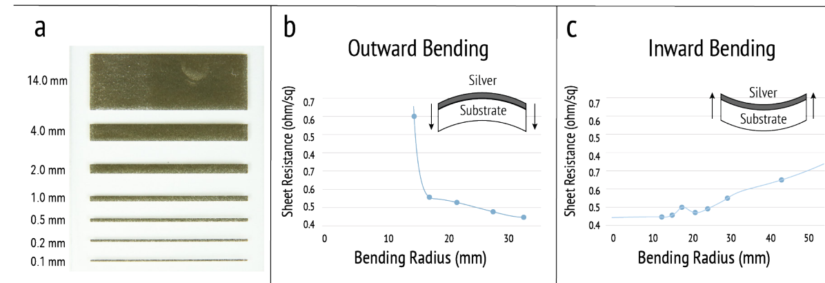
Fig. 7. (a) Transfer resolution. (b) Resistance under outward bending. (c) Resistance under inward bending.
